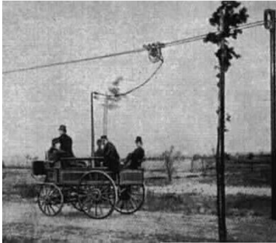
Electromote, Berlin 1882
